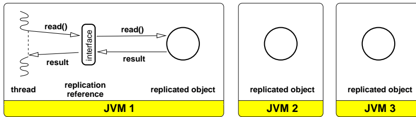
Figure 4.2: A read method is applied on an object replicated on three JVMs.
