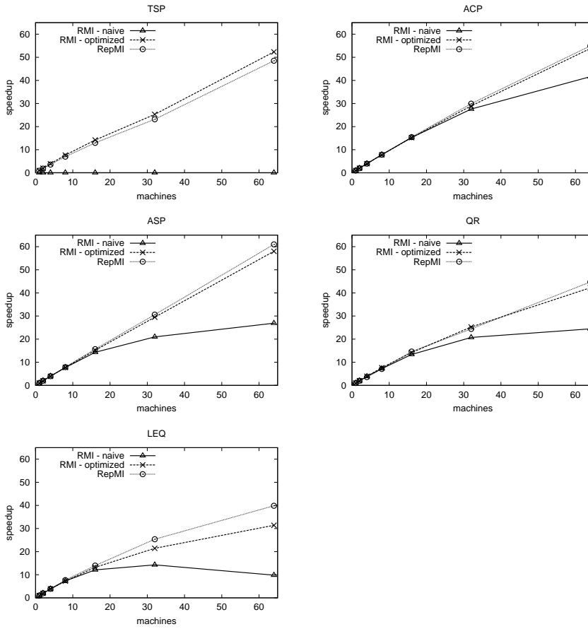
Figure 4.14: Application speedups.
