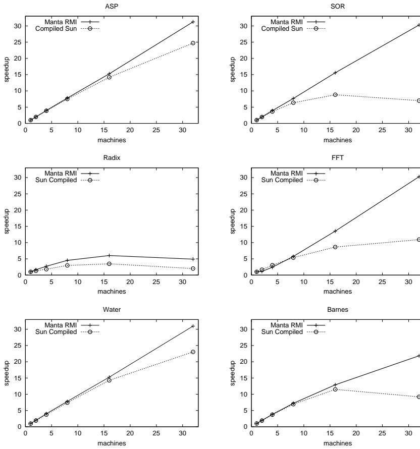
Figure 3.10: Application speedups.
