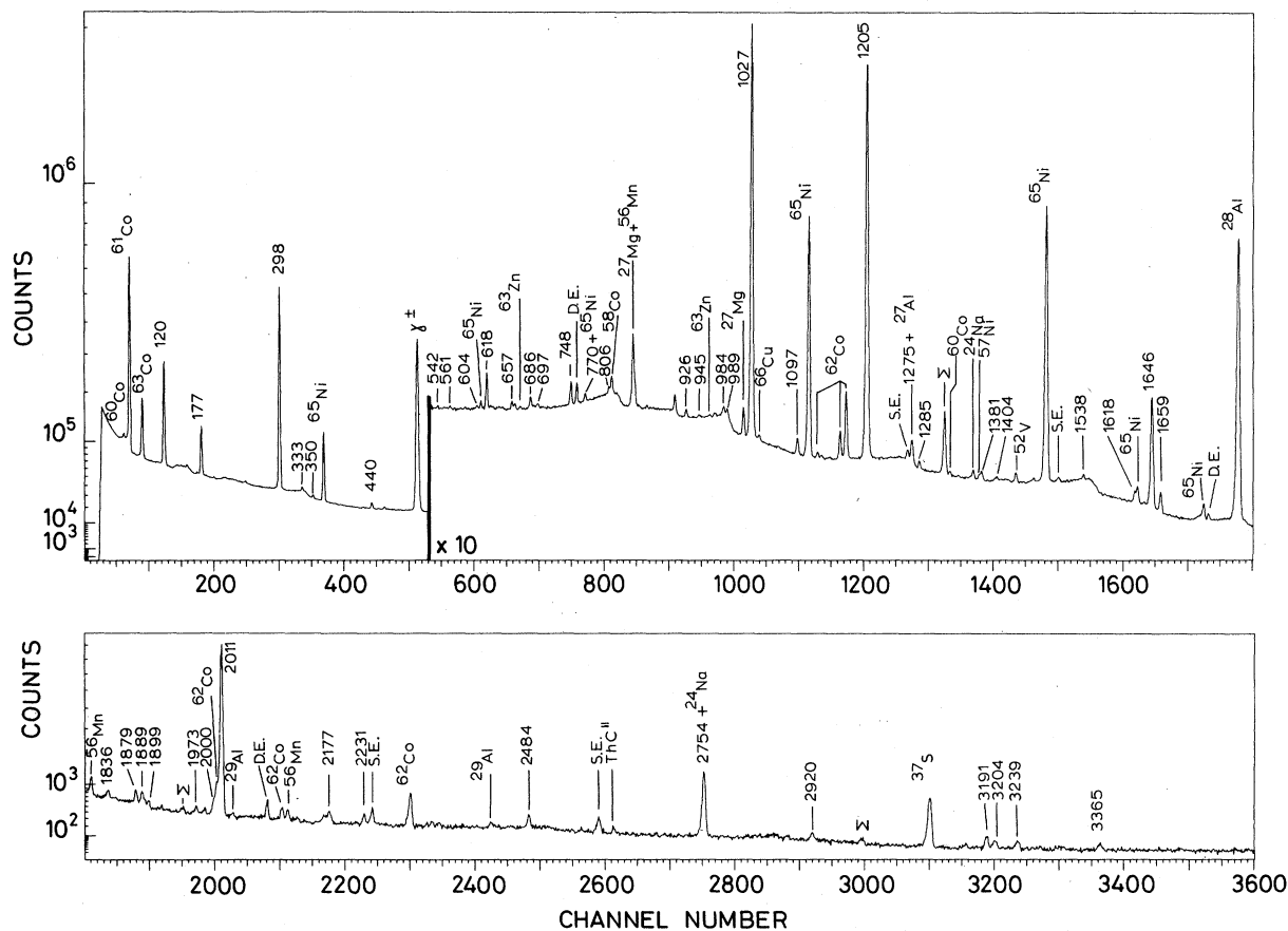
FIG. 1. The \gamma ray spectrum of ^{61}\text{Fe} , obtained by adding the spectra of 25 sources, produced by the AVF cyclotron. Each spectrum was measured during 6 min, starting 0.5 min after the end of irradiation. The \gamma transitions of ^{61}\text{Fe} are indicated with their energies in keV. Peaks due to coincident summation are indicated by a "Σ".
