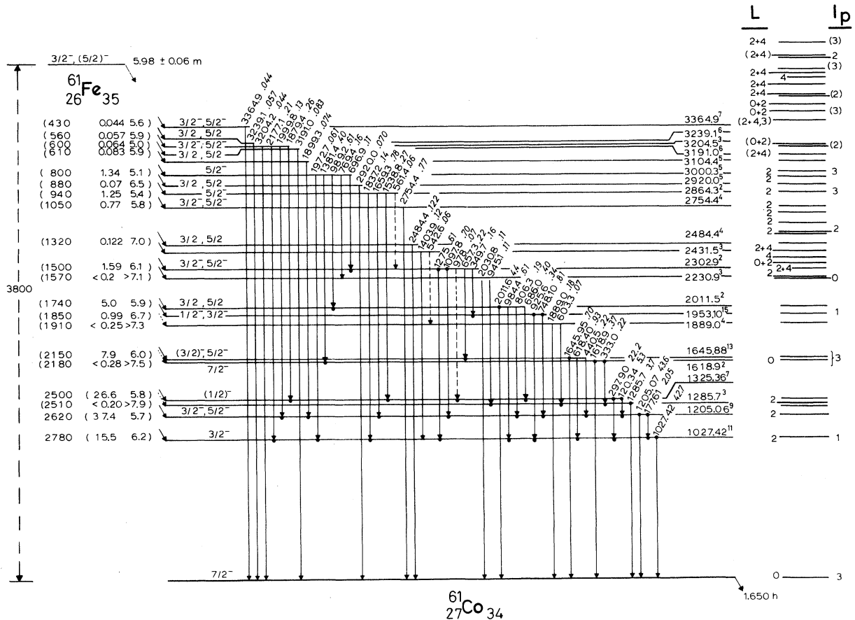
FIG. 4. The proposed decay scheme of ^{61}\text{Fe} . The energies are given in keV. The total decay energy, as well as the decay energies to the 1027.42, 1205.06, and 1325.36 keV levels are taken from Ref. 9. Transition intensities are given in percentage per decay. The \beta feedings are calculated from the relative \gamma intensities. Uncertain \beta feedings have been omitted. The \log ft values are calculated by a program of the Nuclear Data Group. Coincidence relationships which are twice observed are indicated with dots. The level scheme of ^{61}\text{Co} as found in reaction work (Refs. 8, 10, 11, 12) is given on the right, together with the transferred angular momentum in the ^{59}\text{Co}(t, p)^{61}\text{Co} (Ref. 12) reaction ( L ) and in the ^{62}\text{Ni}(t, \alpha)^{61}\text{Co} (Refs. 8 and 9) reaction ( l_p ). The spins of levels in ^{61}\text{Co} are derived by assuming that the g.s. spin of ^{61}\text{Fe} is \frac{3}{2} .
