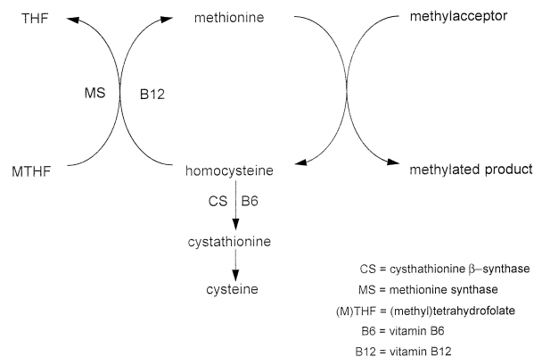
Fig. 1 Methionine–homocysteine metabolism.
